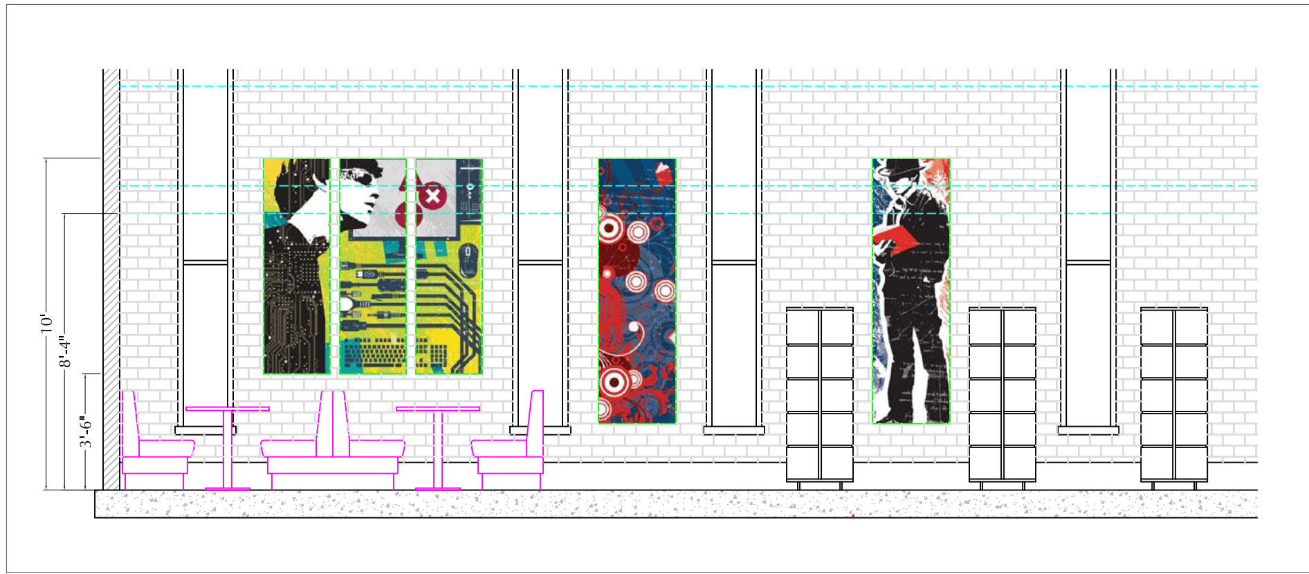
1 A1.2 PRODUCT LAYOUT - PLAN VIEW
